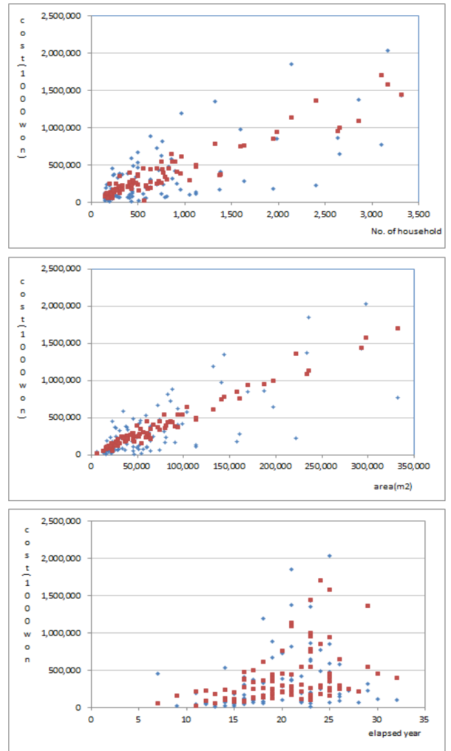
Fig.4. Relation between the repair cost and No. of household, Management Area and Elapsed Year in fully elevator work
