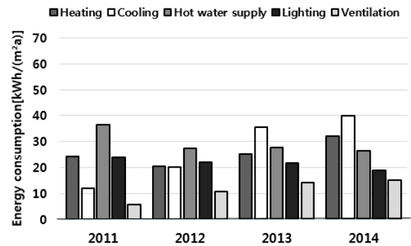
Fig. 11. Itemized energy consumption status
