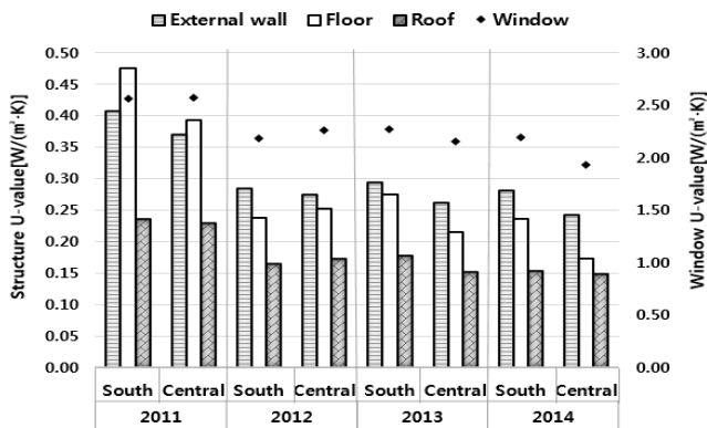
Fig. 2. Envelope U-value status
