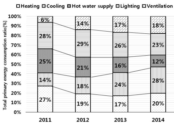
Fig. 12. Itemized total primary energy consumption ratio status
