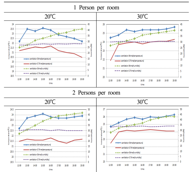
Fig. 4. Temperature and humidity changes
