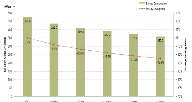
Fig 14. [E Type] of Energy Saving Rate Compared
