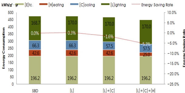
Fig 1. Compare Energy Savings according to the Natural Light
