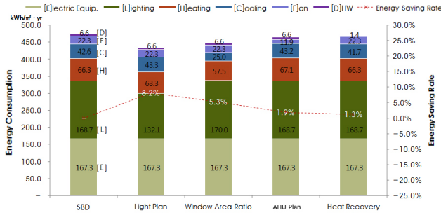
Fig 8 Compare Energy Savings according to Light Plan / Window Area Ratio / Ventilation Plan / Heat Recovery
