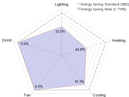
Fig 13. [C Type] Specific Elements Energy Saving Rate
