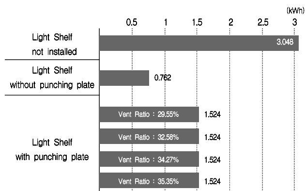
Fig. 7. Consumption of electric power according to types of Light Shelf
