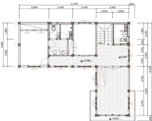
Fig. 5. 2nd Floor Plan
